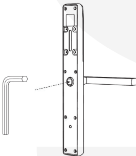
1. Loosen the screw on the Handle (Counterclockwise)
